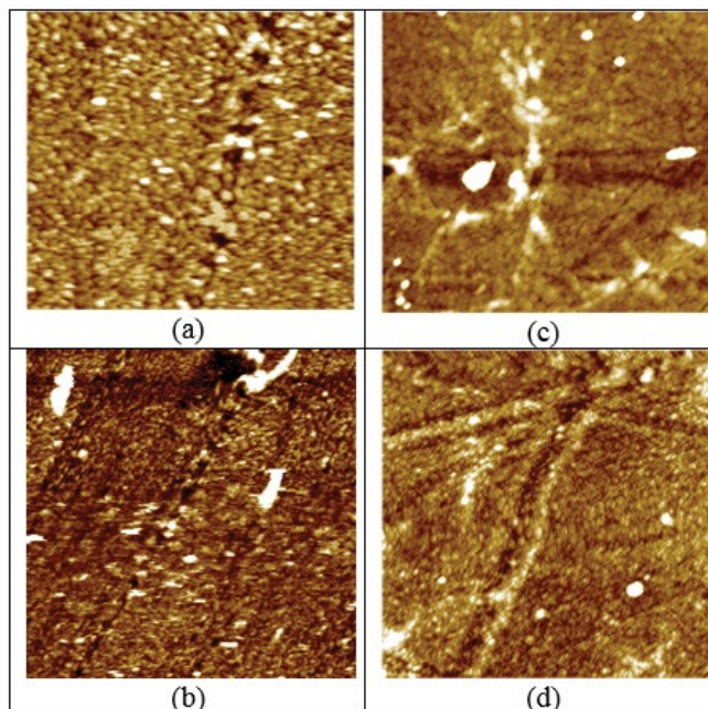
Figure 4: AFM scans of PET samples: (a) treated with an SF_6 plasma (50 mtorr, 100 W, 900 s by PI anode - R = 1.8 nm); (b) treated with an SF_6 plasma (50 mtorr, 100 W, 900 s by PI cathode - R = 4.7 nm); (c) treated with an SF_6 plasma (50 mtorr, 25 W, 900 s by PIII - R = 2.6 nm); (d) treated with an SF_6 plasma (50 mtorr, 100 W, 900 s by PIII - R = 2.5 nm).
