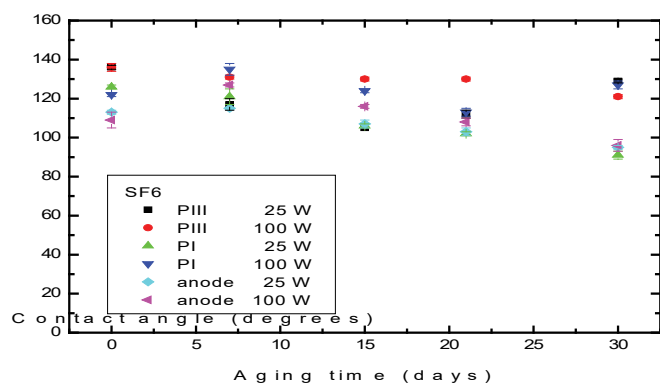
Figure 2: \theta evolution on aging time of PET surfaces that were exposed to SF_6 plasma for 900 s, at 25 W and 100 W of RF Power.
