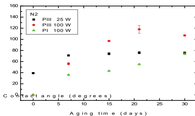
Figure 1: \Theta evolution on aging time of PET surfaces that were exposed to N 2 plasma for 900 s, at 25 W and 100 W of RF Power.
