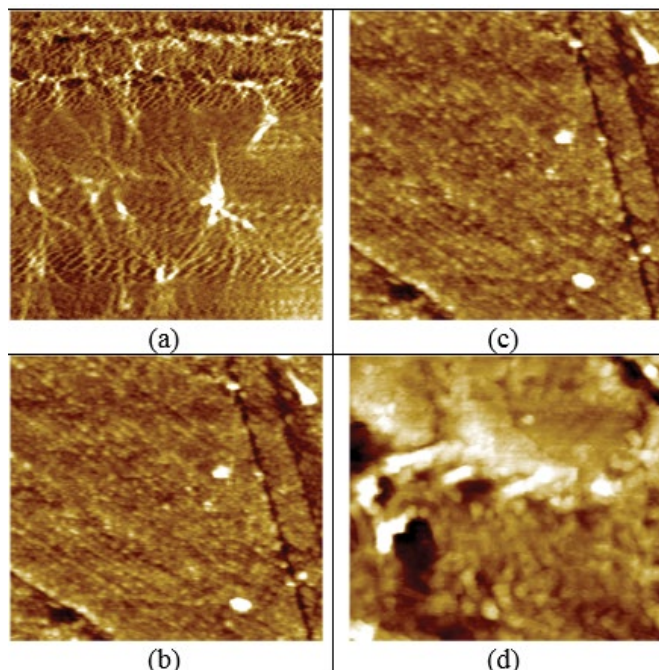
Figure 3: AFM 5 \mu m \times 5 \mu m of scans of PET samples: (a) untreated PET - R = 1.8 nm; (b) treated with N_2 plasma (50 mtorr, 100 W, 900 s by PI cathode - R = 4.4 nm); (c) treated with an N_2 plasma (50 mtorr, 25 W, 900 s by PIII - R = 1.4 nm); (d) treated with N_2 plasma (50 mtorr, 100 W, 900 s by PIII - R = 1.7 nm).
