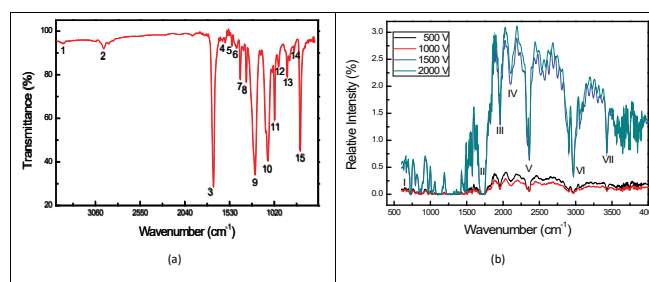
Figure 1: Infrared Spectra of virgin PET for the identification of functional groups in (a) virgin PET (b) implanted PET. The treatment parameters were 13.33 Pa of N 2 for 300 s, at 25 W for different high voltages and a cycle time of 30 μs at 300 Hz.
