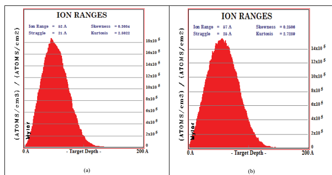
Figure 3: (a) Depth (Angstroms) of incident ions (F + ) for the PET, using incident energy of 1 keV (b) Depth (Angstroms) of incident ions (N + ) for the PET, using incident energy of 1 keV. The histogram represents the range of values average and maximum.
